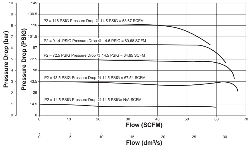
ER09 Regulator 1/4" Ports
