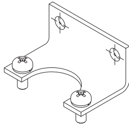
Foot Bracket
