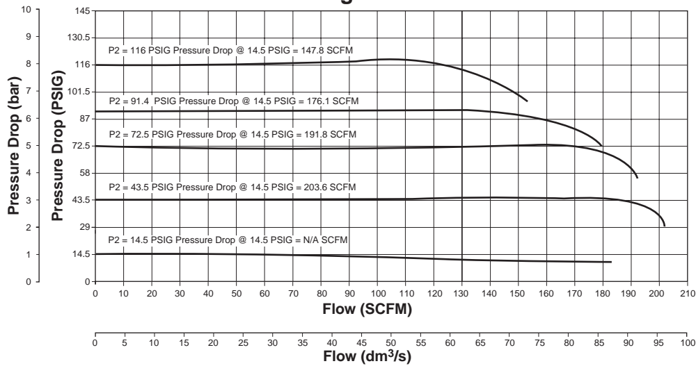
ER19 Regulator 1/2" Ports
