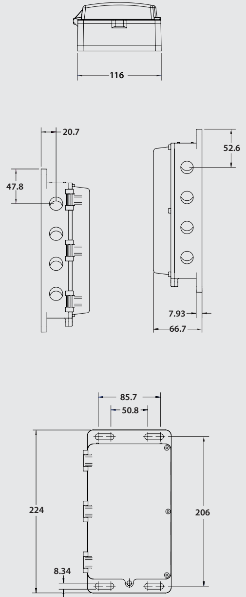
Dimensions (mm)
